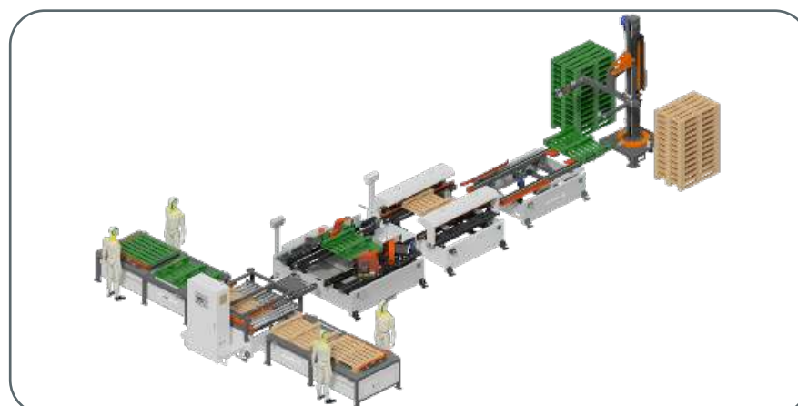
SF9030 Pallet assembly line
